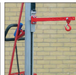
Jib and Hook - EP07 500mm long Capacity: 150kg £195.00
